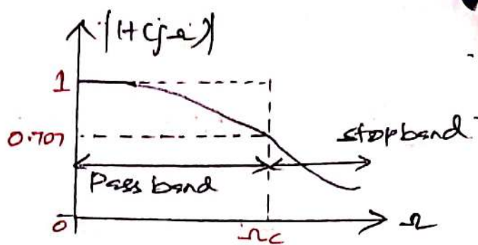
(b) practical lowpass filter
