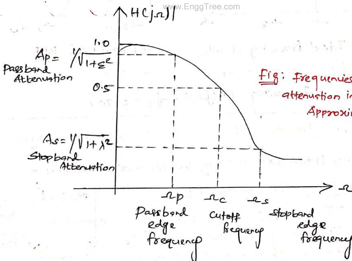
Fig: Butterworth Characteristic
