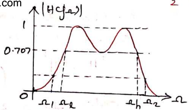
(b) Practical BPF
