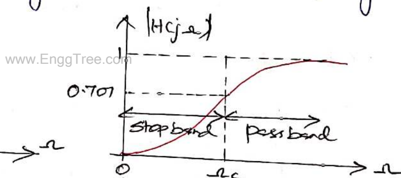
(b) practical HPF
